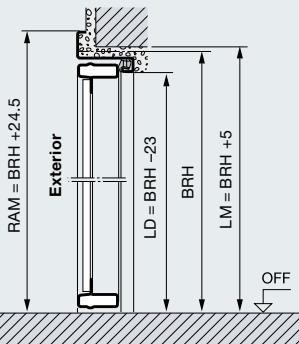
External fitting opening outwards
