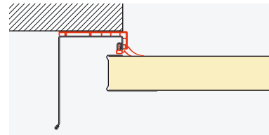
Side sealing
